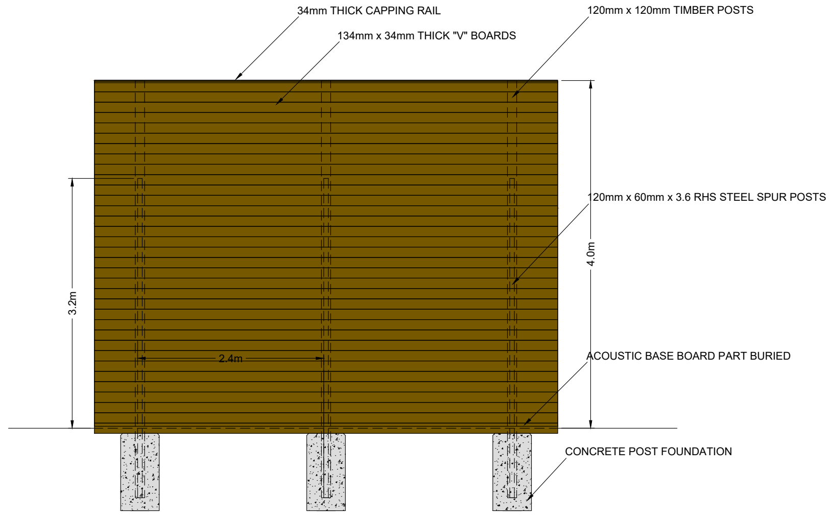
FRONT ELEVATION
