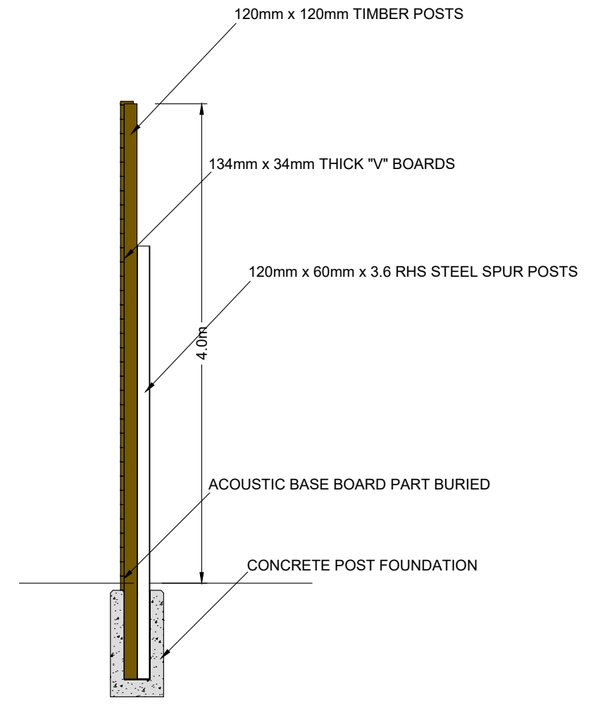
SECTION
