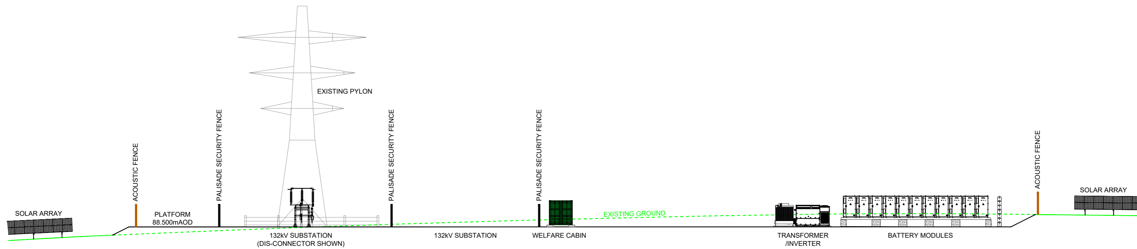
SECTION 1-1
