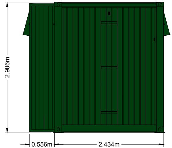
NORTHERN ELEVATION
