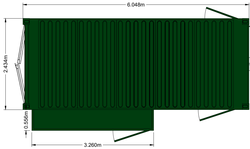
ROOF PLAN
