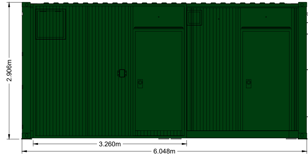
WESTERN ELEVATION
