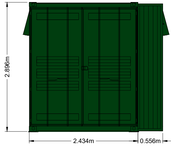
SOUTHERN ELEVATION
